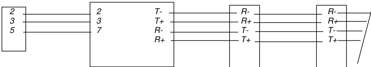
Câble RS232
