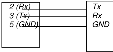
Câble RS232
