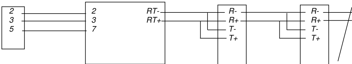
Câble RS232
