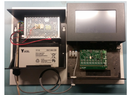
Example of connection between Battery backup and FG-NET digital unit
